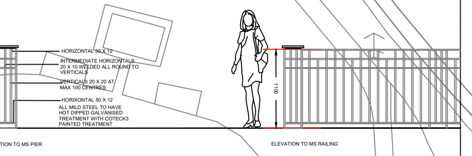
MILD STEEL RAILING TO PLAY AREA
