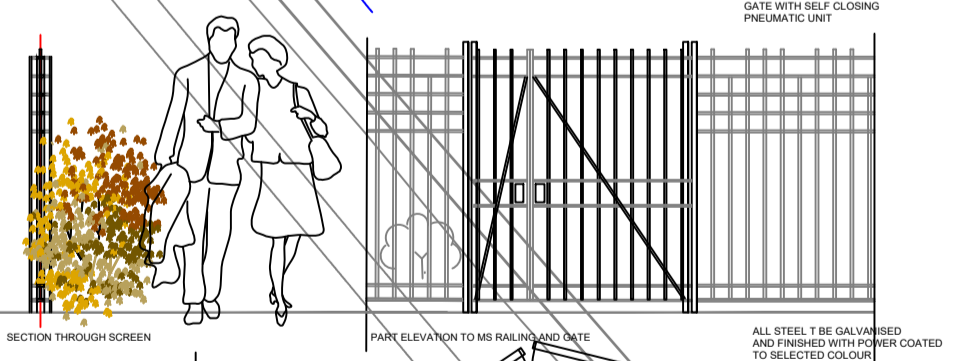
MILD STEEL RAILING 1.5 M HIGH WITH SELF CLOSING GATES
